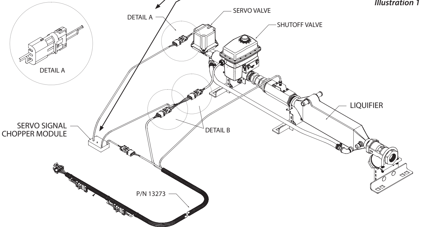
NH3 System Diagram after Servo Signal Chopper Module Installation
